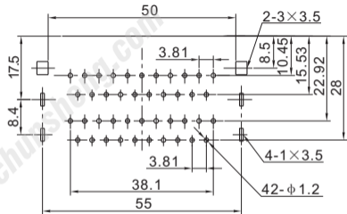
P.C.B LAYOUT (VIEWED FROM COPPER SIDE)
