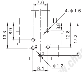
P.C.B LAYOUT (VIEWED FROM COPPER SIDE)
