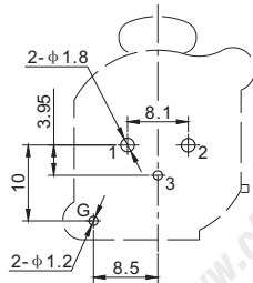
P.C.B LAYOUT (VIEWED FROM COPPER SIDE)
