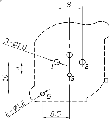
P.C.B. LAYOUT (Tolerance: ±0.1) (BOTTOM VIEW)
