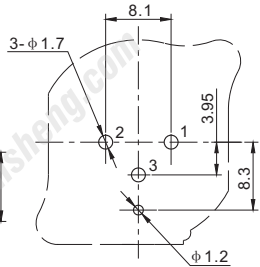
P.C.B LAYOUT (VIEWED FROM COPPER SIDE)
