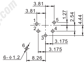
P.C.B LAYOUT (VIEWED FROM COPPER SIDE)
