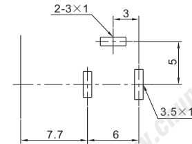
P.C.B LAYOUT (VIEWED FROM COPPER SIDE)
