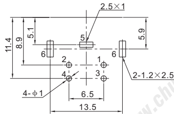
P.C.B LAYOUT (VIEWED FROM COPPER SIDE)
