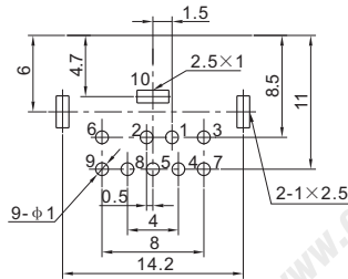
P.C.B LAYOUT (VIEWED FROM COPPER SIDE)
