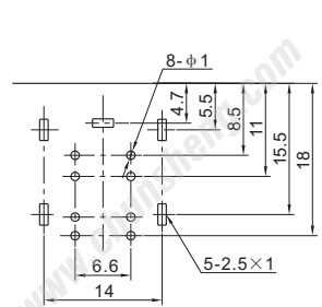
P.C.B LAYOUT (VIEWED FROM COPPER SIDE)
