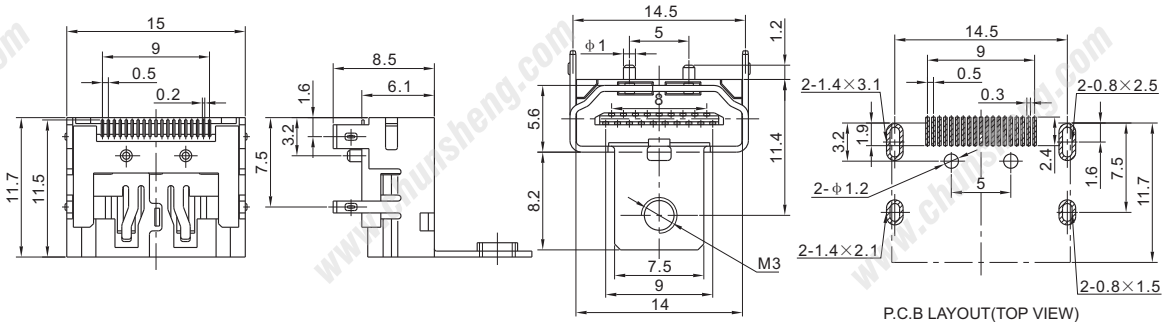
HDMI-AF-002
