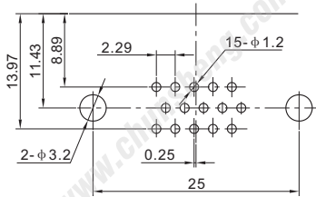
P.C.B LAYOUT (VIEWED FROM COPPER SIDE)
