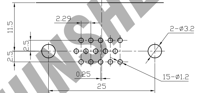
PCB MOUNTING HOLES (VIEWED FROM COPPER SIDE)
