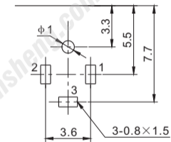
P.C.B LAYOUT (VIEWED FROM COPPER SIDE)
