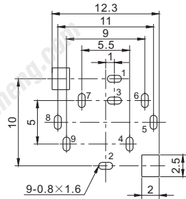
P.C.B LAYOUT (VIEWED FROM COPPER SIDE)
