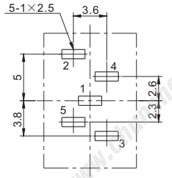
P.C.B LAYOUT (VIEWED FROM COPPER SIDE)
