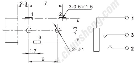
P.C.B LAYOUT (VIEWED FROM COPPER SIDE)
