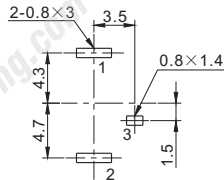
P.C.B LAYOUT (VIEWED FROM COPPER SIDE)
