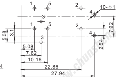
P.C.B LAYOUT (VIEWED FROM COPPER SIDE)
