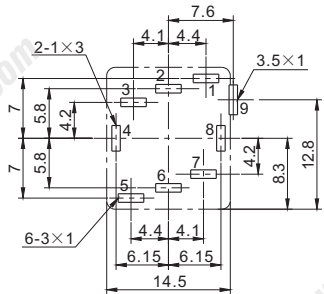
P.C.B LAYOUT (VIEWED FROM COPPER SIDE)
