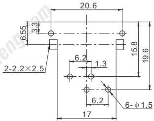
P.C.B LAYOUT (VIEWED FROM COPPER SIDE)
