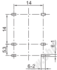
P.C.B LAYOUT (VIEWED FROM COPPER SIDE)
