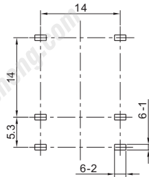
P.C.B LAYOUT (VIEWED FROM COPPER SIDE)
