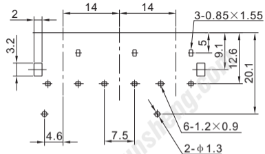
P.C.B LAYOUT (VIEWED FROM COPPER SIDE)
