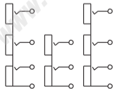
P.C.B LAYOUT (VIEWED FROM COPPER SIDE)
