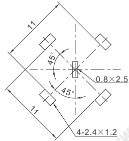
P.C.B LAYOUT (VIEWED FROM COPPER SIDE)
