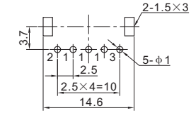
P.C.B LAYOUT (VIEWED FROM COPPER SIDE)
