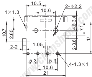
P.C.B LAYOUT (VIEWED FROM COPPER SIDE)
