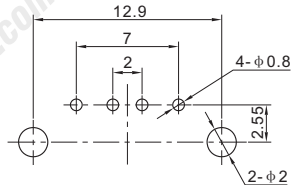
P.C.B LAYOUT (VIEWED FROM COPPER SIDE)
