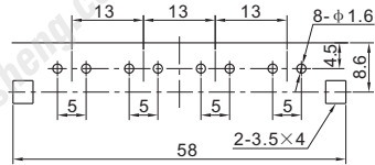
P.C.B LAYOUT (VIEWED FROM COPPER SIDE)
