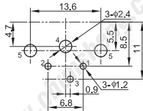
PCB LAYOUT (TOP VIEW)
