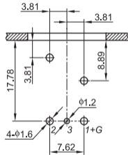
PCB LAYOUT (TOP VIEW)
