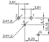
PCB LAYOUT (TOP VIEW)
