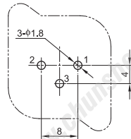
PCB LAYOUT (TOP VIEW)
