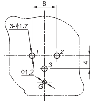
PCB LAYOUT (TOP VIEW)
