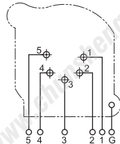
PCB LAYOUT (TOP VIEW)
