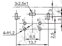
PCB LAYOUT (TOP VIEW)
