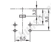
PCB LAYOUT (TOP VIEW)
