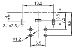
PCB LAYOUT (TOP VIEW)
