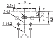
PCB LAYOUT (TOP VIEW)
