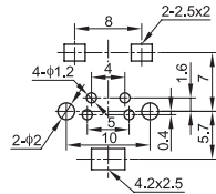
PCB LAYOUT (TOP VIEW)
