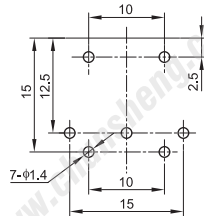
PCB LAYOUT (TOP VIEW)
