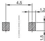
PCB LAYOUT (TOP VIEW)
