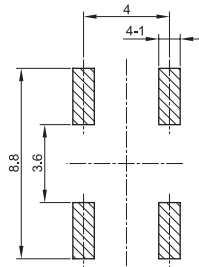
PCB LAYOUT (TOP VIEW)
