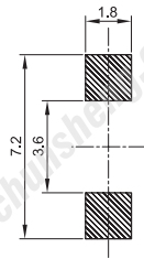
PCB LAYOUT (TOP VIEW)
