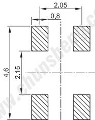
PCB LAYOUT (TOP VIEW)
