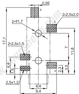
PCB LAYOUT (TOP VIEW)
