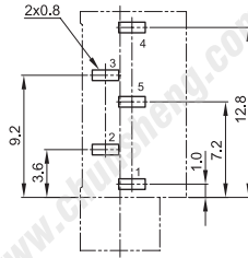
PCB LAYOUT (TOP VIEW)
