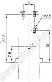
PCB LAYOUT (TOP VIEW)
