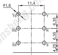
PCB LAYOUT (TOP VIEW)
