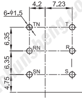
PCB LAYOUT (TOP VIEW)
